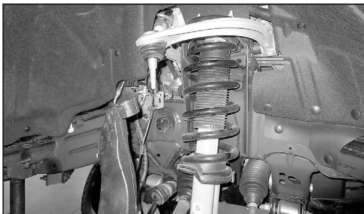
FIGURE 8 - STEP 7
