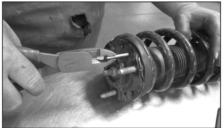
FIGURE 10 - STEP 10
