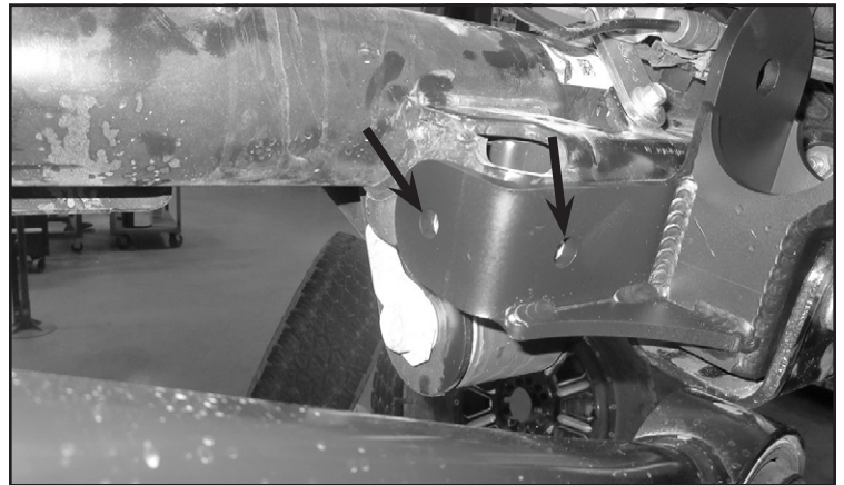
FIGURE 24 - STEP 36
